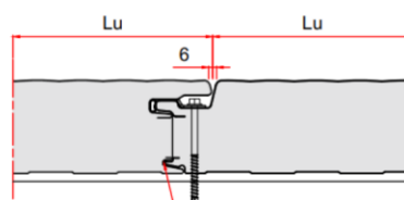
Figure 5 – Panneau sandwich isolant KS 600/900/1000 CX
