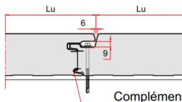
Figure 1 – Panneau sandwich isolant KS 600/900/1000 FL-S
