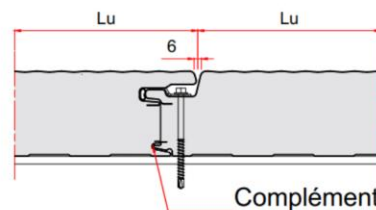
Figure 2 – Panneau sandwich isolant KS 600/900/1000 MR
