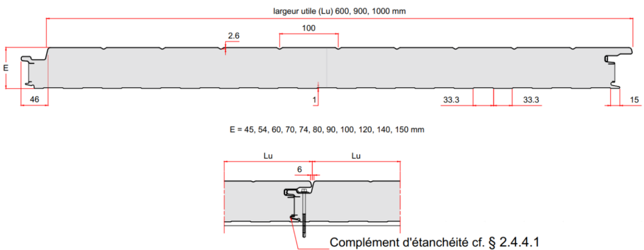
Figure 7 – Panneau sandwich isolant KS 600/900/1000 PL
