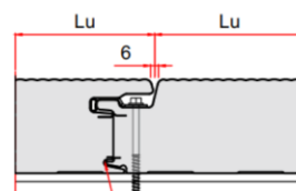
Figure 3 – Panneau sandwich isolant KS 600/900/1000 MM
